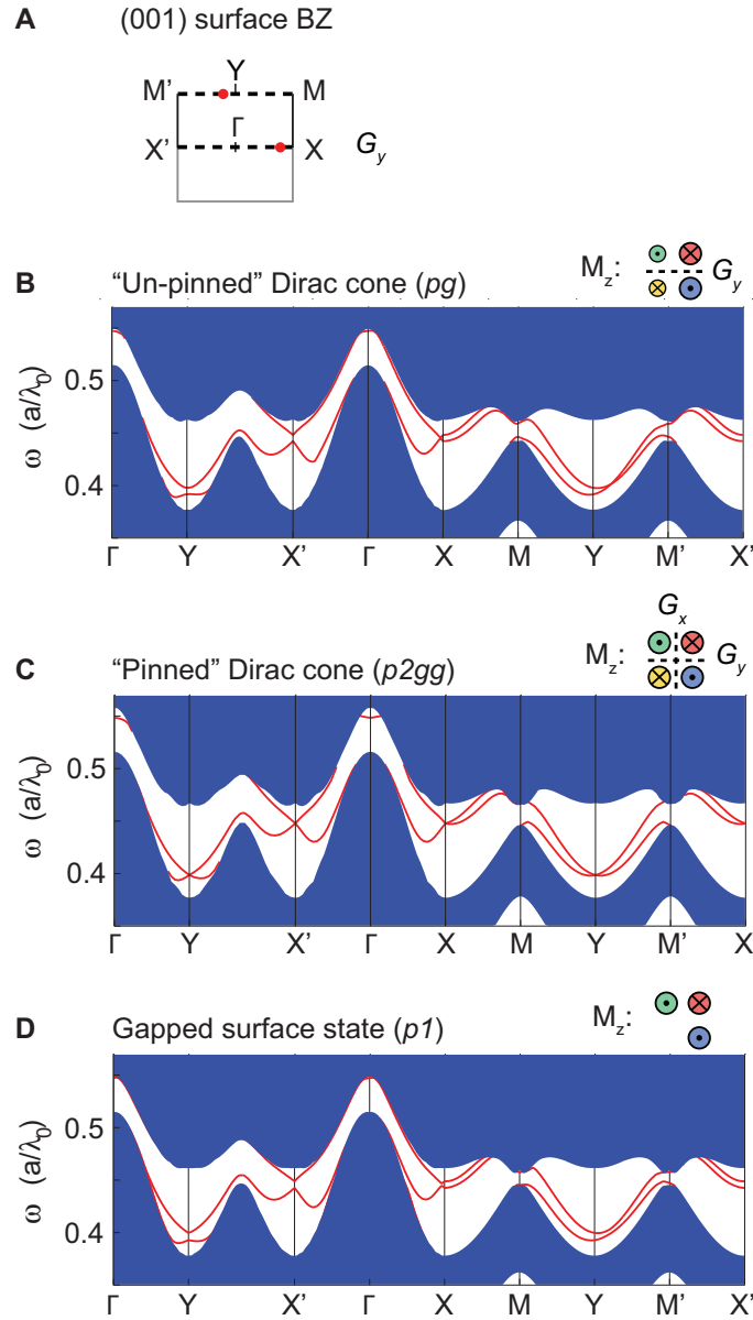
FIG. S1: The (001) surface states after breaking \mathcal{T} . A) (001) surface Brillouin zone. B) Single Dirac cones un-pinned along X-X' and M-M' lines protected by one glide reflection ( G_y ). C) Single Dirac cones pinned at X and Y points by the extra glide ( G_x ). D) Single Dirac cones are gapped due to the loss of glide reflections 3 . A perfect metallic boundary is placed from top, at the center of the cubic cell, on the (001) surface with an air gap spacing of 0.4a from the photonic crystal surface.
