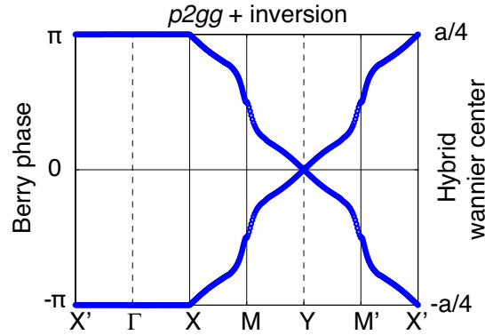
FIG. S3: The gapless hybrid Wannier centers corresponds to the non-trivial surface states ( p2gg ) in Fig. 2C.
