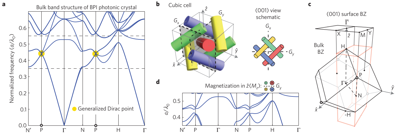
Figure 1 | BPI photonic crystal. a , Bulk band structure of the BPI photonic crystal in the bcc lattice. The GDP is between the first four bands. b , Cubic unit cell of length a consisting of four identical dielectric rods oriented along the bcc lattice vectors of (111) (red), (1\bar{1}\bar{1}) (yellow), (\bar{1}11) (blue) and (\bar{1}\bar{1}1) (green). The rods go through (0, 0, 0)a , (0, 0.5, 0)a , (0.5, 0, 0)a and (0, 0, 0.5)a , respectively. There are two glide reflection planes ( G_x and G_y ) in the structure, invariant on the (001) surface. The top-view schematic illustrates the relations between the rods under operations of G_x and G_y . c , The bcc BZ and its projection onto the (001) surface BZ. The transparent red box outlines the volume in the bulk BZ that projects to half of the surface BZ. d , Bulk band structure showing that the GDP opens when magnetization is applied on the rods without breaking G_y .
