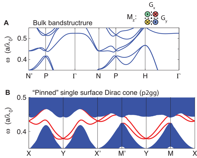
FIG. S2: Bulk and surface band structures of ferrimagnetic (gyromagnetic) photonic crystals. A) Bulk band structure showing the gap opening of the GDP. B) Gapless Z_2 surface states of single Dirac cones at X \equiv X' and Y \equiv Y' . A perfect metallic boundary is placed from top, at the center of the cubic cell, on the (001) surface with an air gap spacing of 0.4a from the photonic crystal surface.
